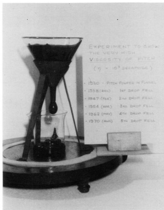
Figure 1 Apparatus for the pitch drop experiment showing the dates of each event. See also table 1.
